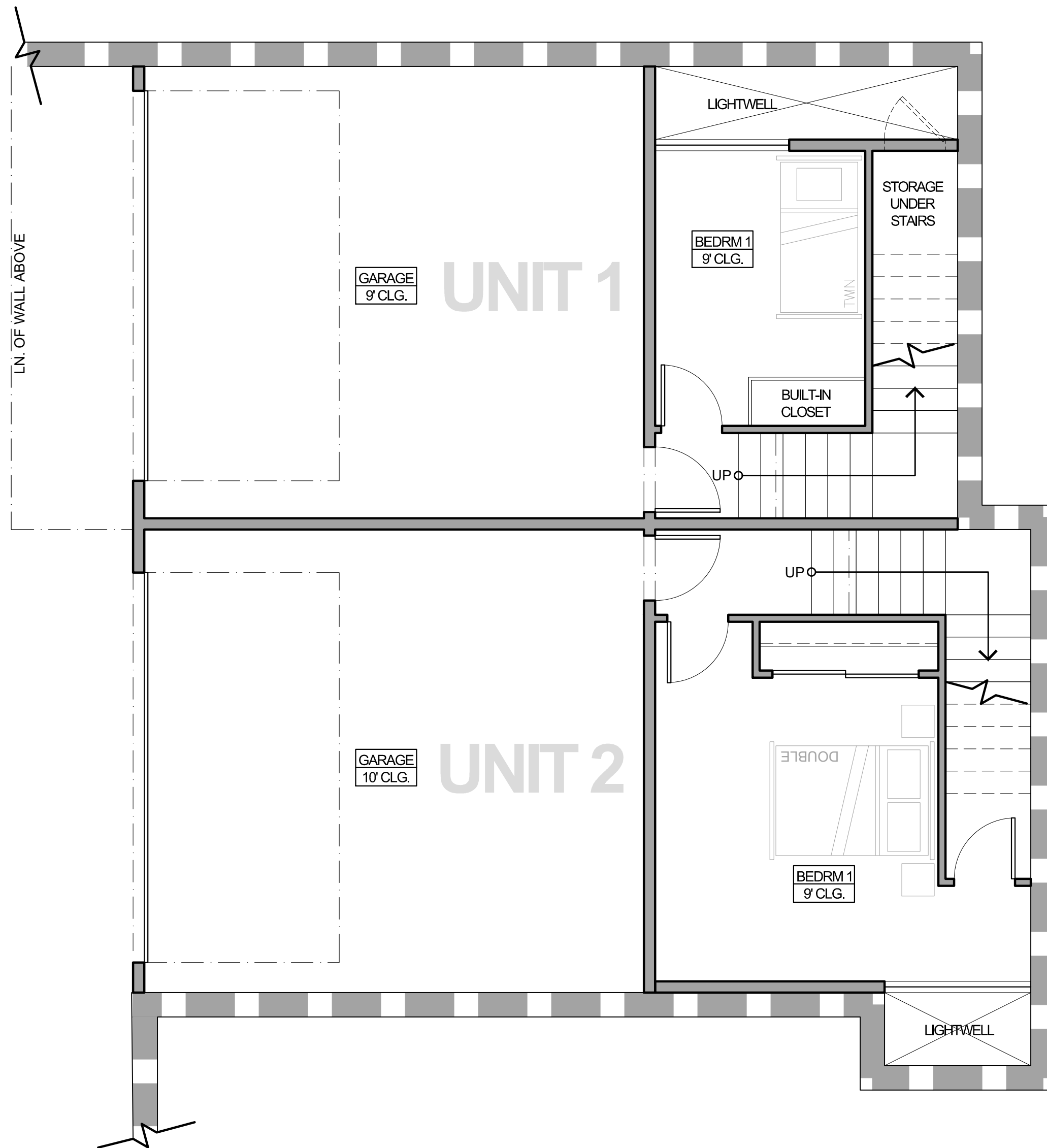
BASEMENT FLOOR PLAN 1/4" = 1'-0"
