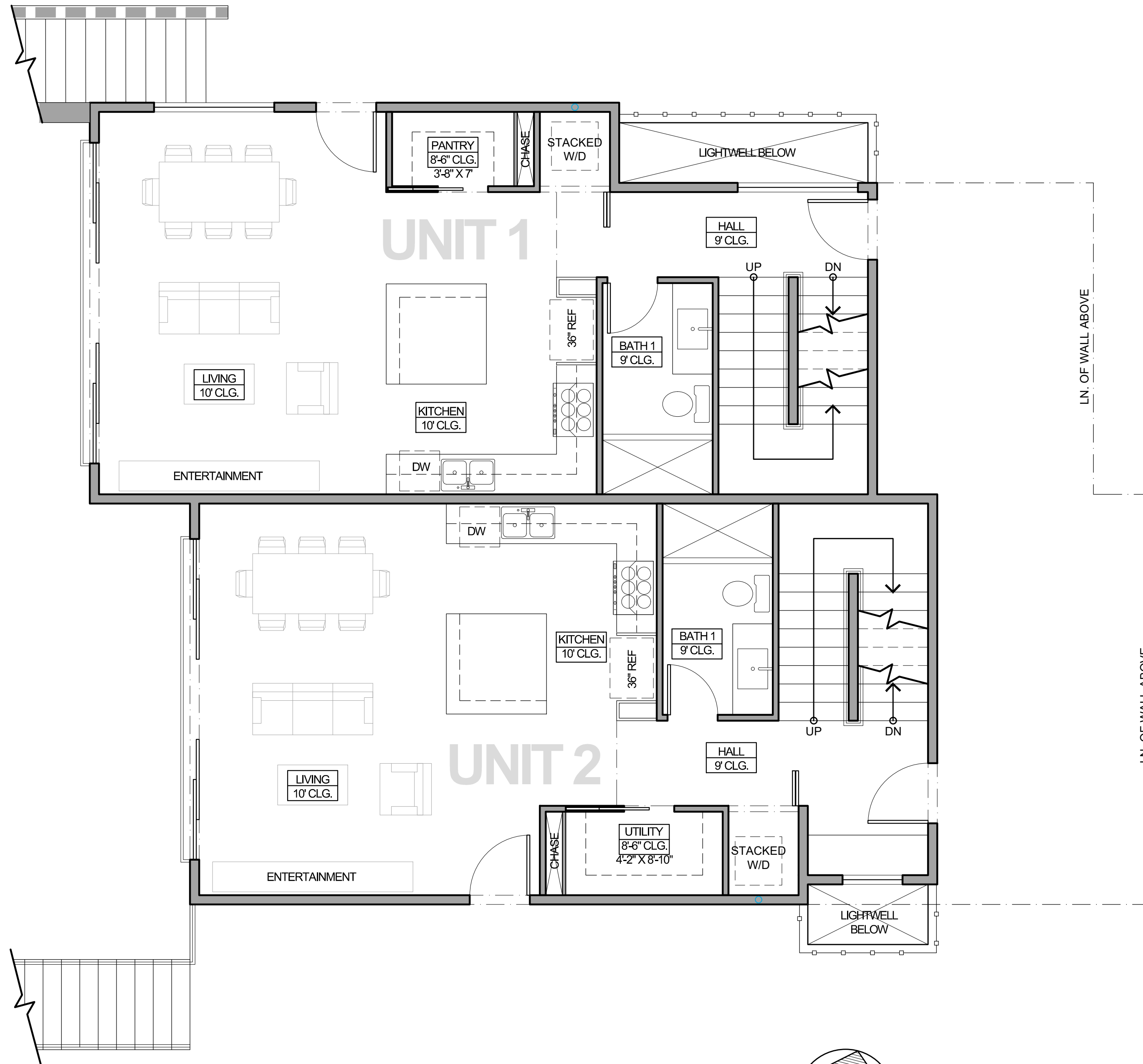
MAIN FLOOR PLAN 1/4" = 1'-0"
